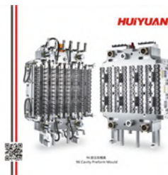
96CAVITY PREFORM MOULD Product neck :Pco 1881 Product weight :22.7g Match machine: Husky Hypet-400
