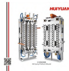
48 CAVITY PREFORM MOULD Product Neck:29/25 Product weight :12.5g0
