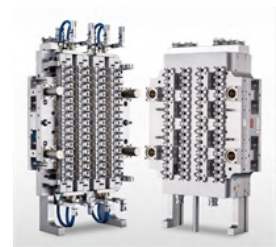
64CAVITY PREFORM MOULD Product Neck:29/25 Product weight :11.8g
